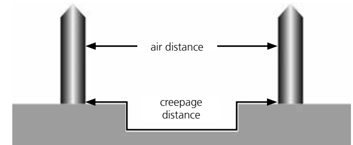
Fig 2. Isolation coordination
